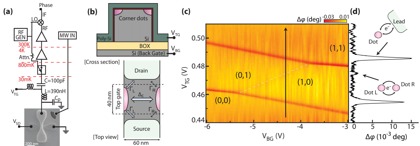
FIG. 1. Dispersive detection of a DQD. (a) Scanning electron microscope image of a device connected to an rf-reflectometry setup via the top gate. A nearby on-PCB coplanar waveguide delivers MW signals. (b) Device schematic. Top: cross section perpendicular to current flow direction, indicating the location of the corner QDs, where BOX indicates the buried oxide layer. Bottom: top view of the device, with transparent top gate for clarity; five electronic transitions between dots and reservoirs marked by arrows. \Delta_c represents the tunnel coupling and \Gamma_{L(R)} the relaxation rates between the left (right) dot and the reservoirs. (c) Resonator phase response \Delta\phi as a function of top-gate and back-gate voltages ( V_{TG} , V_{BG} ). The white dashed line emphasizes the ICT and the black solid arrow indicates the position of the trace in panel (d). DQD electron numbers appear in parentheses. (d) \Delta\phi as a function of V_{TG} , showing the relative intensity of the ICT and the DST.
