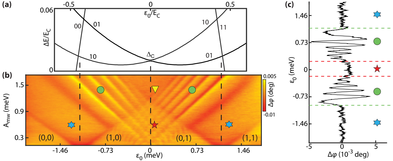
FIG. 3. Multilevel LZSM interferometry. (a) Calculated DQD energy level diagram as a function of reduced detuning \epsilon_0/E_C ; \alpha_- = 0.05 and E_m/E_C = 10 , where E_m is the mutual charging energy. (b) \Delta\phi measured as a function of the detuning, \epsilon_0 , and MW amplitude, A_{mw} , for f_{mw} = 21 GHz. Regions of constant \Delta\phi , with well-defined electron numbers, are indicated in parentheses. The (10)-(01) anticrossing and the (00)-(10) and (01)-(11) crossings are indicated by black dashed lines. Incoherent, multipassage, double-passage, and single-passage LZSM regions are indicated by the blue star, red star, green circle, and yellow triangle, respectively. (c) \Delta\phi vs \epsilon_0 trace at A_{mw} = 0.55 meV and f_{mw} = 11 GHz. Symbols as in (b).
