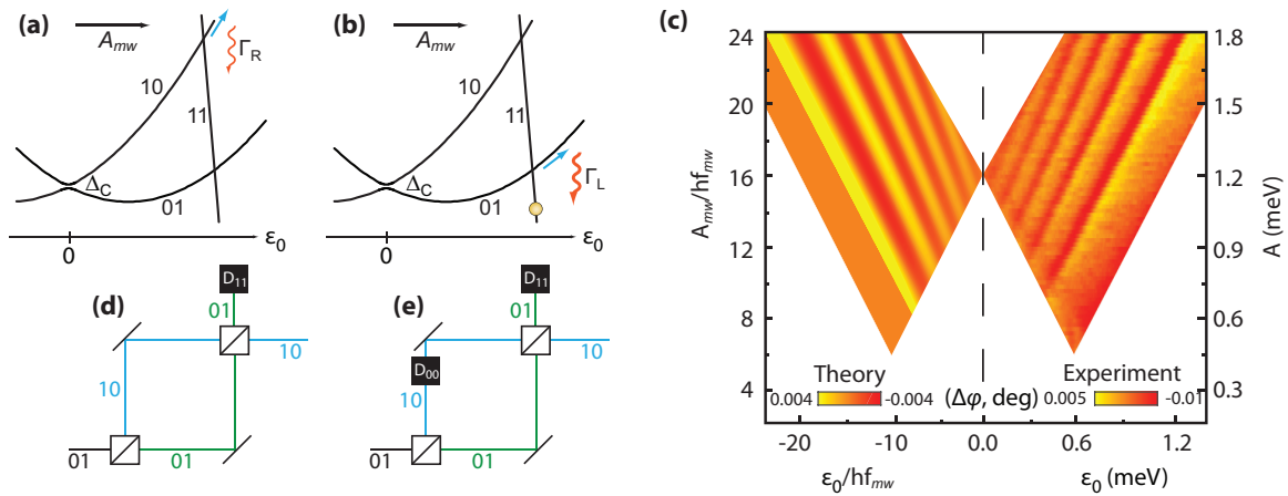
FIG. 4. Double-passage LZSM interferometry. LZ transition schematic at the (10)-(11) (a) and (01)-(11) (b) crossings. The blue arrow indicates P_{LZ} \approx 1 and the red arrow thickness shows the strength of the relaxation process. (c) \Delta\phi calculated (left) vs experimental [right, a section of Fig. 3(b)]. (d) Optical interferometry analog now including the detector D_{11} after the second passage [fast relaxation at the (01)-(11) transition]. (e) Optical interferometry analog for the single-passage regime including an additional detector D_{00} after the first passage [relaxation at the (10)-(00) transition].
