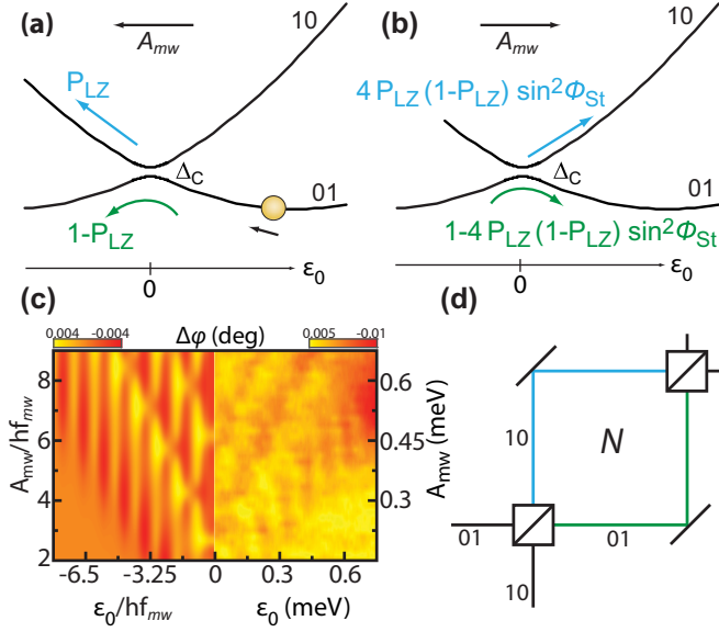
FIG. 2. Multipassage LZSM interferometry. Schematic of the probability distribution after the first (a) and second (b) passage. (c) \Delta\varphi calculated (left of panel) vs experimental (right of panel), both panels mirrored in the horizontal direction with respect to one another. (d) Optical interferometry analog showing the photon paths (electron charge states), the beam splitters (fast passage through the anticrossing), and refocusing mirrors (microwave electric fields). Here the process is repeated N times.
