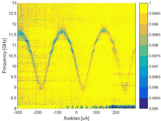
Fig. 2. The measured transmission through the cavity with 21X21 SQUIDs array versus frequency and versus external magnetic field. The probing RF signal power level is set low enough (-70 dBm) in order to keep the response linear (RF power independent). The data shows a possibility of 21X21 SQUID array tuning in 8-12.5 GHz range. The resonance response of SQUID array seems to be synchronous, with no additional branches (parasitic resonances) visible, as for a singular RF SQUID, with periodical variation of resonance frequency versus magnetic field.
