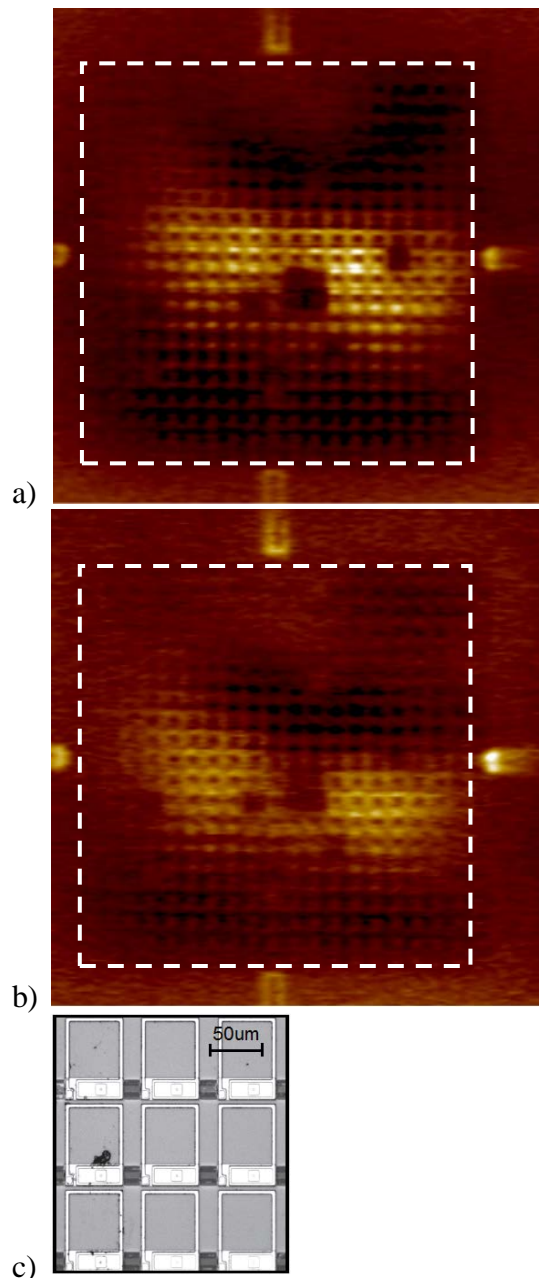
Fig. 3. LSM generated images of the RF currents in the 21 X 21 SQUIDs array at the RF frequency close to the maximum resonance frequency of SQUIDs (Fig. 2). (a, b) LSM data at F_{max} - two independent measurements. In figures the light color coding corresponds to the maximum of LSM response, showing the area with the superconductive circuit with the strongest RF current. The dotted line shows the limit of the SQUID filled area of about 1 X 1 mm. (c) optical image of close up view of 9 SQUIDs in the tested array, about 1/50 of the total area. The two dark spots in the center of views a) and b) (no RF currents) are likely to be the two defective SQUIDs. One can note that about 50 % of the SQUIDs in the array participating in the resonance (bright color). The remaining question of the resonance modal structure in the SQUID array requires RF phase information unavailable in LSM experiments.
