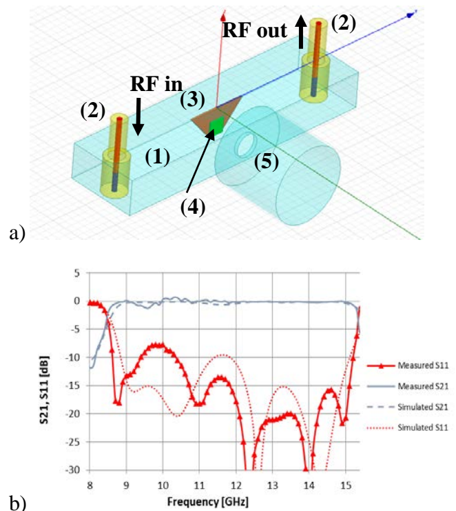
Fig. 1 a) The waveguide chamber used for cryogenic test of RF SQUID metasurface. In the sketch is shown a section of the 19 mm X 9.5 mm waveguide (1). The waveguide section is terminated with the two waveguide-to-coaxial adapters (2) letting the RF signal in and out of the chamber, and the sample mounting plate (3) in the center. When the SQUID array is mounted at the support plate (3) the sample (4) is getting installed inside of the waveguide facing the optical window (5). The window (5) lets in the waveguide the optical probing beam of the Laser Scanning Microscope and is not transparent for the RF probing signal. b) The measured (solid line) and HFSS simulated (dotted line) transmission and reflection coefficients of the test chamber versus frequency of the probing RF signal show the convenience of the developed chamber for the SQUID metasurface characterization in the 8.5 – 15.5 GHz band.
