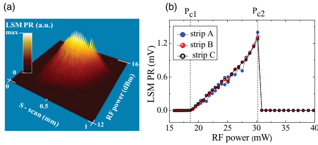
FIG. 4. (Color online) (a) 3D LSM image showing the power dependence of PR_{IL} over the S -line scan shown in Fig. 3(a). (b) Experimental LSM PR vs P_{rf} on a linear scale, taken at three neighboring strips (strip B is located at the center of the S -line scan between strip A and strip C). Both data are obtained at a temperature well below T_c , 4.5 K.
