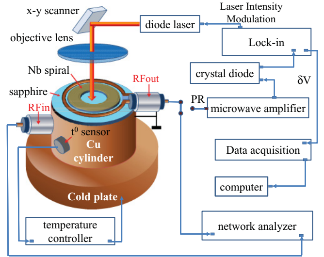
FIG. 2. (Color online) Simplified schematic representation of the LSM setup used for 2D visualization of microwave photoresponse of the tested resonator structure. Drawing is not to scale.
