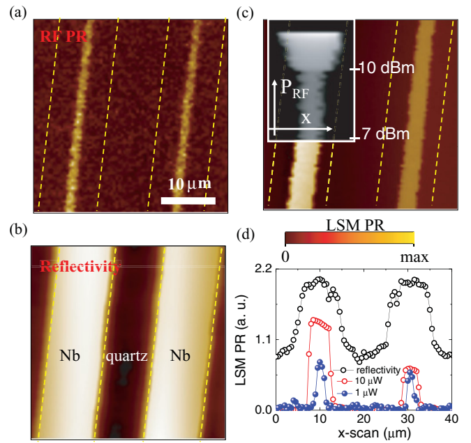
FIG. 5. (Color online) 2D LSM (a) PR_{IL} and (b) reflectivity images taken from 40 \times 40 \mu\text{m}^2 area on the Nb spiral resonator at a laser power of about 1 \mu\text{W} . (c) 2D LSM PR_{IL} image at 10 \mu\text{W} . Inset shows rf power dependence of LSM PR_{IL} on the same area, showing the J_{rf} profiles at low and high rf stimulus. The x -line cut is at the same location in the figure and inset. (d) LSM PR coming from two neighboring Nb turns at two different laser powers; 1 \mu\text{W} and 10 \mu\text{W} . The data are taken at P_{rf} = 7 dBm.
