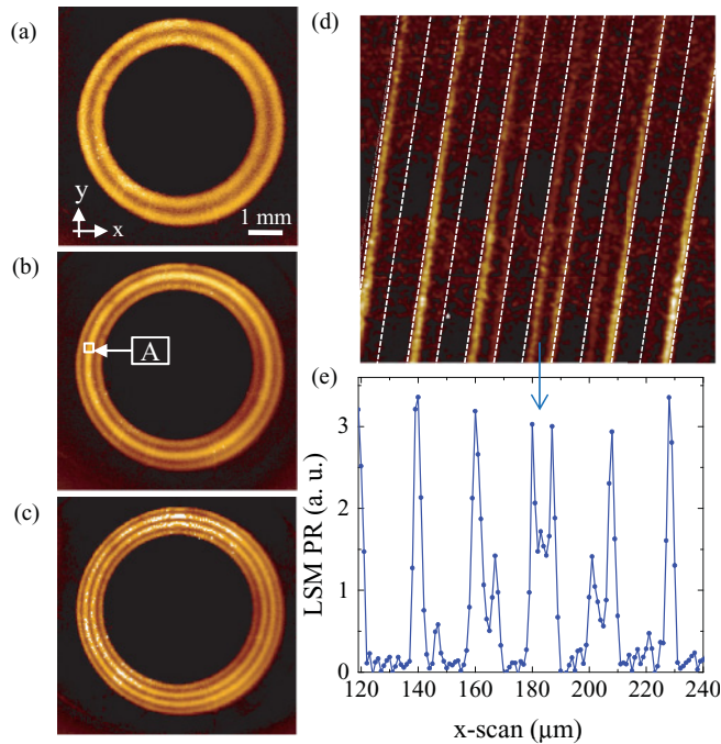
FIG. 7. (Color online) Large-scale 7 \times 7 \text{ mm}^2 LSM PR images showing rf current induced dissipation in a Nb spiral at 4.5 K, 10 dBm and at (a) the second harmonic (219 MHz), (b) the third harmonic (355 MHz), and (c) the fourth harmonic (498 MHz). The area marked A in (b) indicates the position of a detailed 2D image (d) that shows the same rf dissipation in a 125 \times 125 \mu\text{m}^2 region localized at the center of the 3\lambda/2 standing wave pattern. (e) LSM PR profile along a 125\text{-}\mu\text{m} x scan corresponding to the bottom line-scan in (d).
