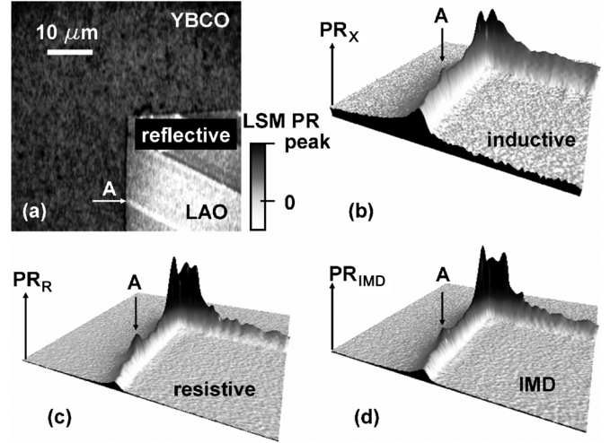
Fig. 3. 2-D LTLSM images of (a) reflectivity map showing the twinned structure of the substrate along with distribution of (b) inductive, (c) resistive, and (d) IMD components of LSM PR obtained in the same 50 \mu\text{m} \times 50 \mu\text{m}^2 area around the inner corners of the resonator structure.
