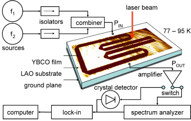
Fig. 1. Schematic of the microwave LSM experiment.
