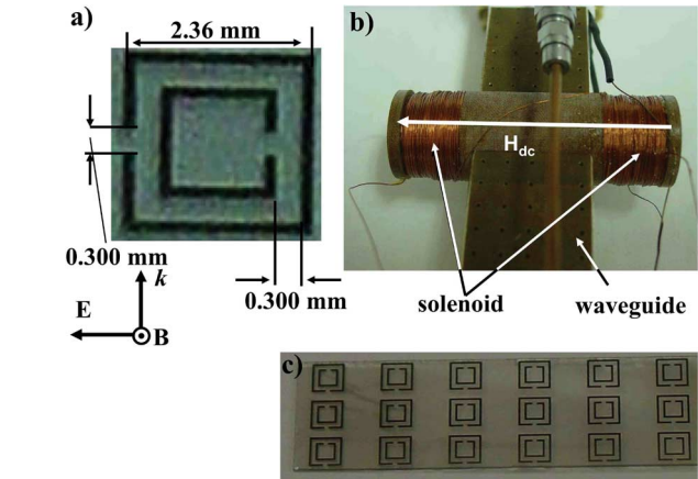
Fig. 1. Images of the materials: (a) Nb (and \text{YBa}_2\text{Cu}_3\text{O}_{7-\delta} ) SRR dimensions and the applied field geometry inside the Ag-plated Cu X-band waveguide; (b) the solenoid straddling the Ag-plated Cu X-band waveguide used in the dc magnetic field experiment; (c) Nb SRR array on a quartz chip.
