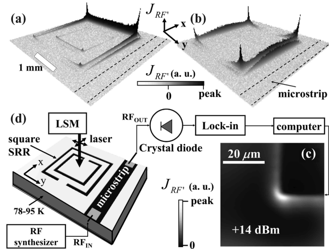
Fig. 6. Laser microscope photoresponse imaging for a single \text{YBa}_2\text{Cu}_3\text{O}_{7-\delta} SRR at 80 K. Part (a) shows J_{\text{RF}'} [11] for the fundamental mode; (b) shows the second harmonic. Part (c) shows J_{\text{RF}'} for a closeup of an inside corner of the inner ring, at 9.57 GHz, and part (d) shows the experimental setup.
