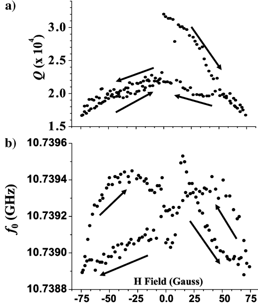
Fig. 3. Measurements of the single Nb SRR in an applied dc H field, at 4.2 K. Arrows indicate direction of field ramping. Part (a) shows the change in Q and part (b) shows the change in the resonant frequency with applied dc H field.
